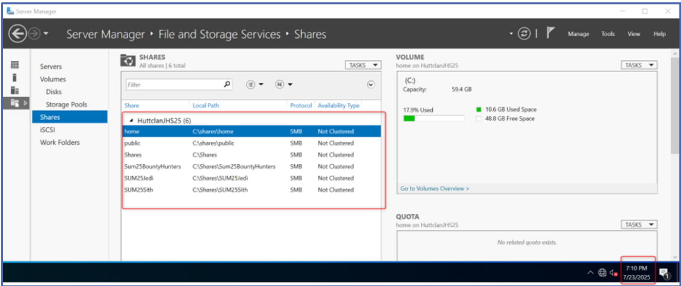
Figure 11 Shared folders on File Server
