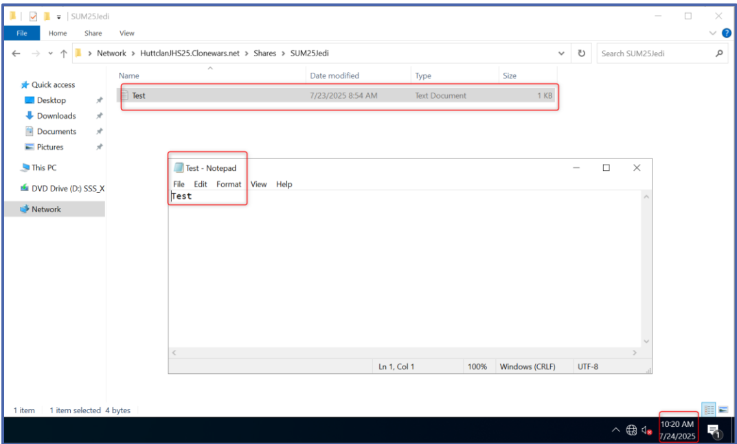
Figure 10 Document Created on Client Opened on File Server
