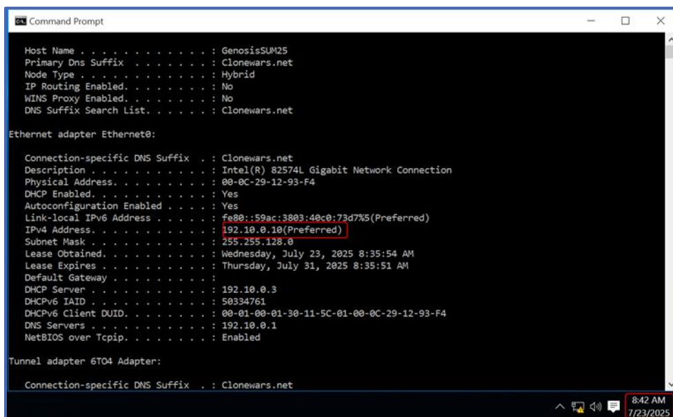
Figure 21 Client Machine DHCP
