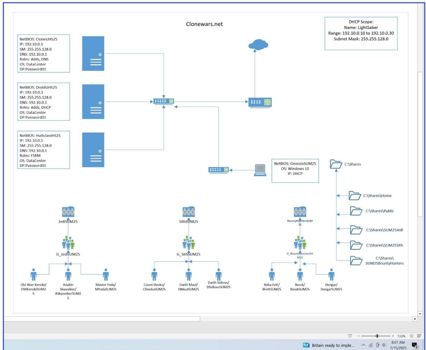
Figure 1 Network and AD DS Diagram
