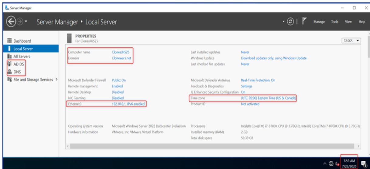
Figure 2 ADDS Server Configuration
