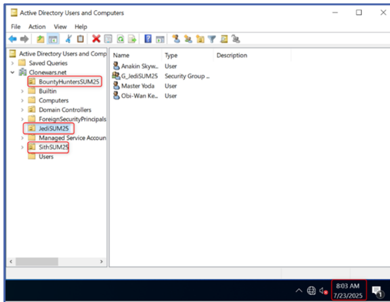
Figure 12 Organizational Units
